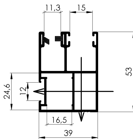
Coulisse A20 (6-001926-xxxx) Sectra
