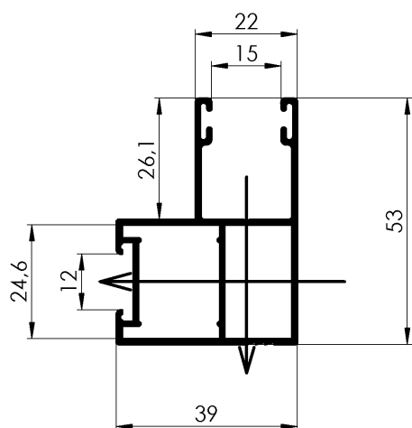
Coulisse A15 (6-001794-xxxx)
