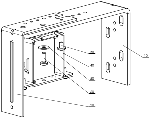
Support réglable double – fixe 206 – 268 mm P 010/45 (2-01803-0000)
